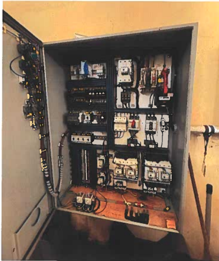
Controller
